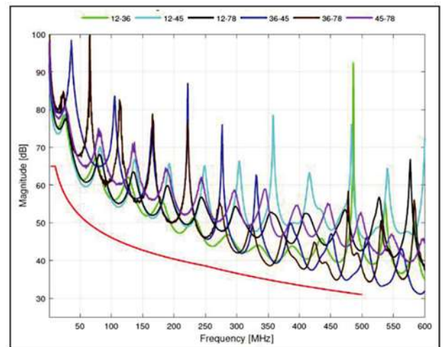
Typical NEXT CAT.6A UTP patch cord
