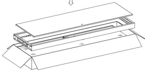
Package A (top cover, bottom plate, shelf, horizontal bracket, accessories)
